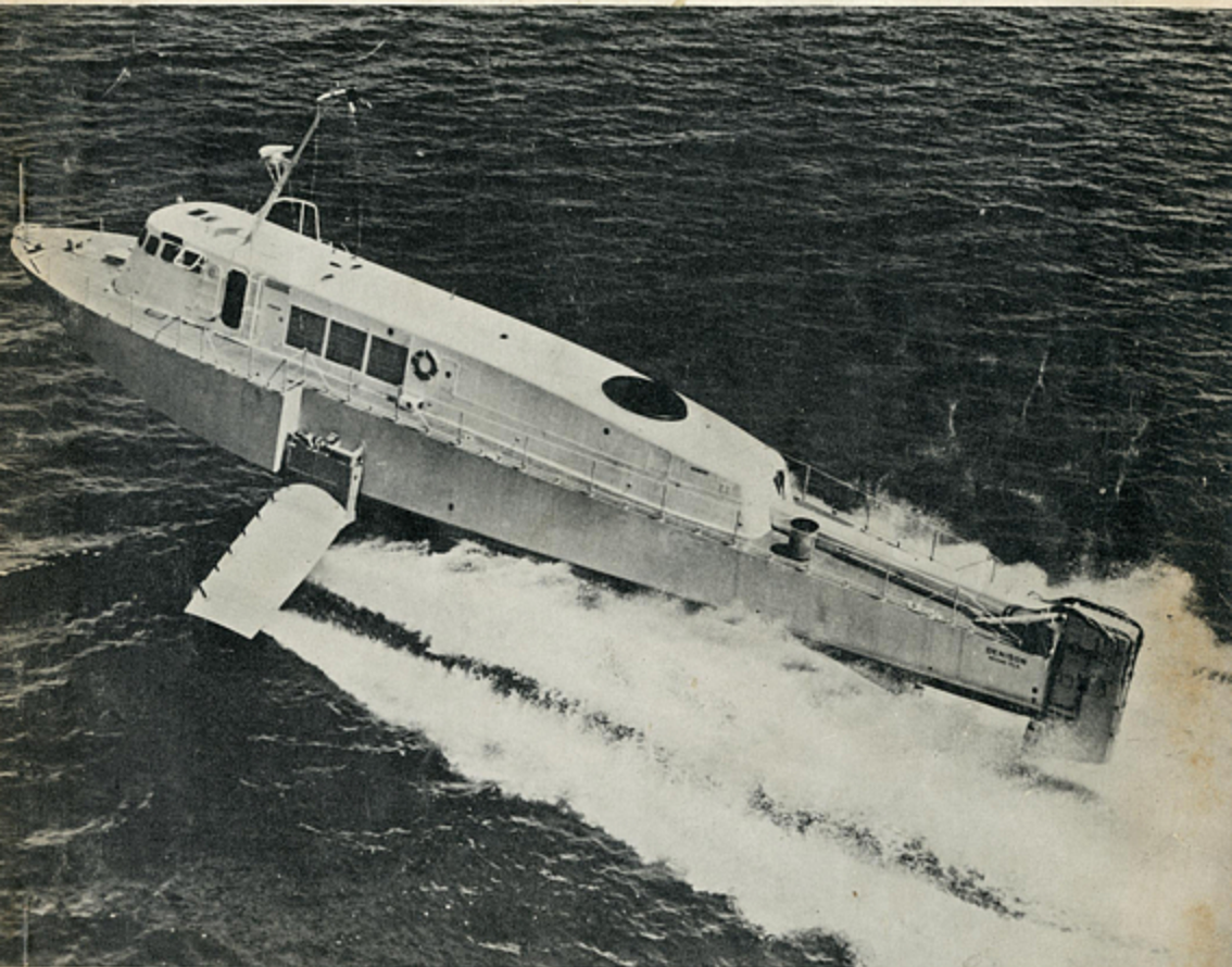
U.S. Hydrofoil Ship Denison at Full Speed
