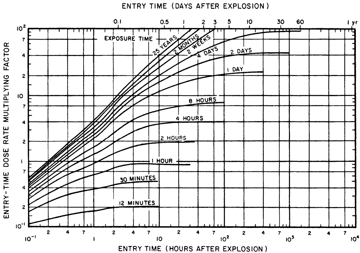
Figure 9.27. Curves for calculating accumulated radiation dose from early fallout based on dose rate at time of entry.
