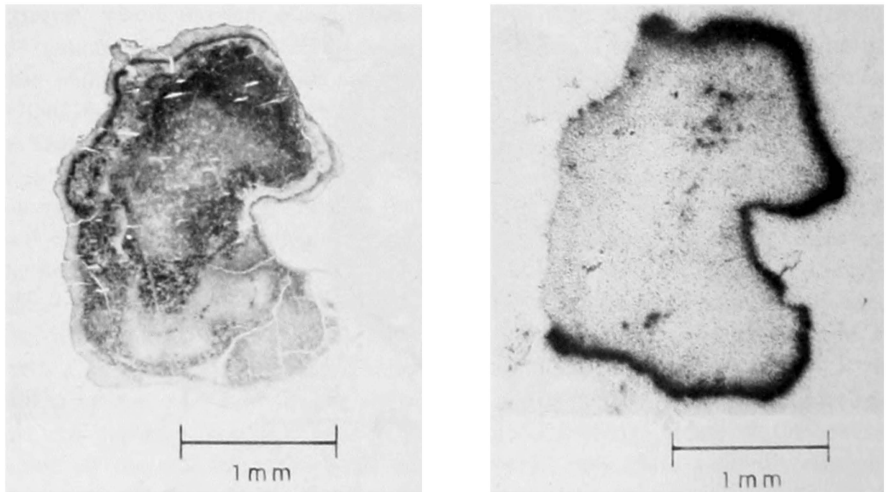
Figure 9.50d. Photograph (left) and autoradiograph (right) of a thin section of an irregular particle from a ground-surface shot at Bikini. The radioactivity is concentrated on the surface of the particle.
