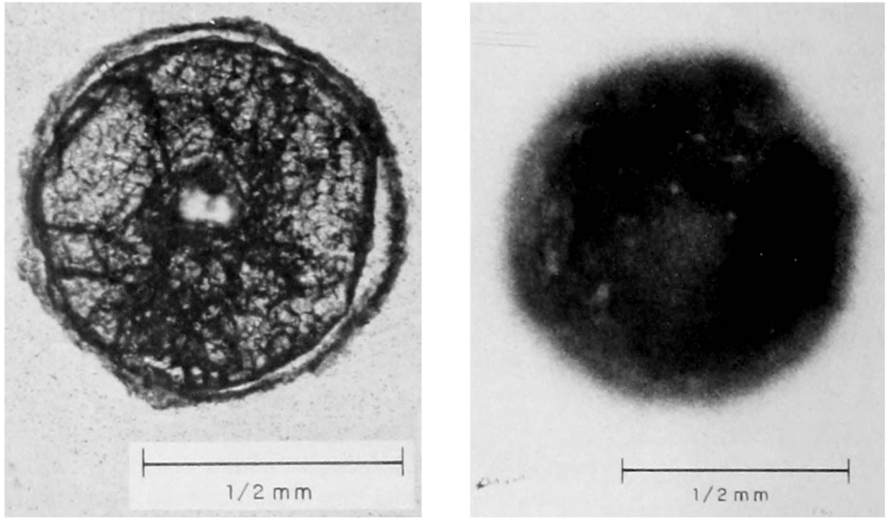
Figure 9.50c. Photograph (left) and autoradiograph (right) of a thin section of a spherical particle from a ground-surface shot at Eniwetok. The radioactivity is uniformly distributed throughout the particle.
