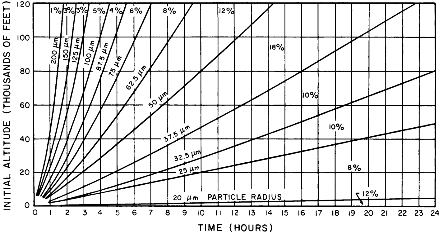
Figure 9.164. Times of fall of particles of different sizes from various altitudes and percentages of total activity carried.
