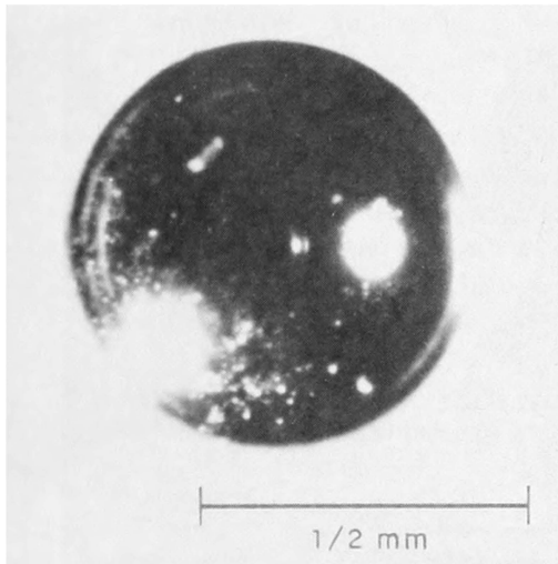
Figure 9.50b. A fallout particle from a tower shot in Nevada. The particle is spherical with a brilliant, glossy surface.
