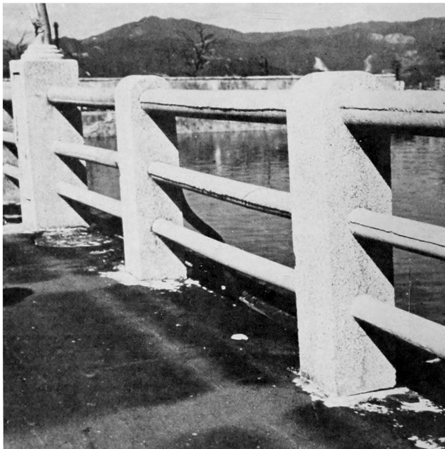
Figure 7.45a. Flash marks produced by thermal radiation on asphalt of bridge in Hiroshima. Where the railings served as a protection from the radiation, there were no marks; the length and direction of the "shadows" indicate the point of the bomb explosion.
