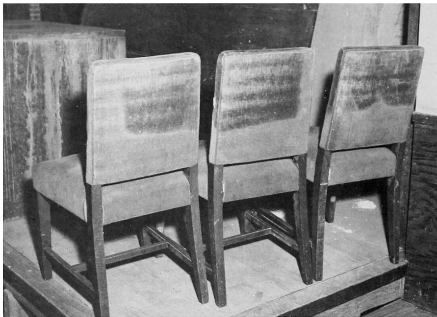
Figure 7.44a. Flash burns on upholstery of chairs exposed to bomb flash at window (1 mile from ground zero at Hiroshima, 8 to 9 cal/cm 2 ).
