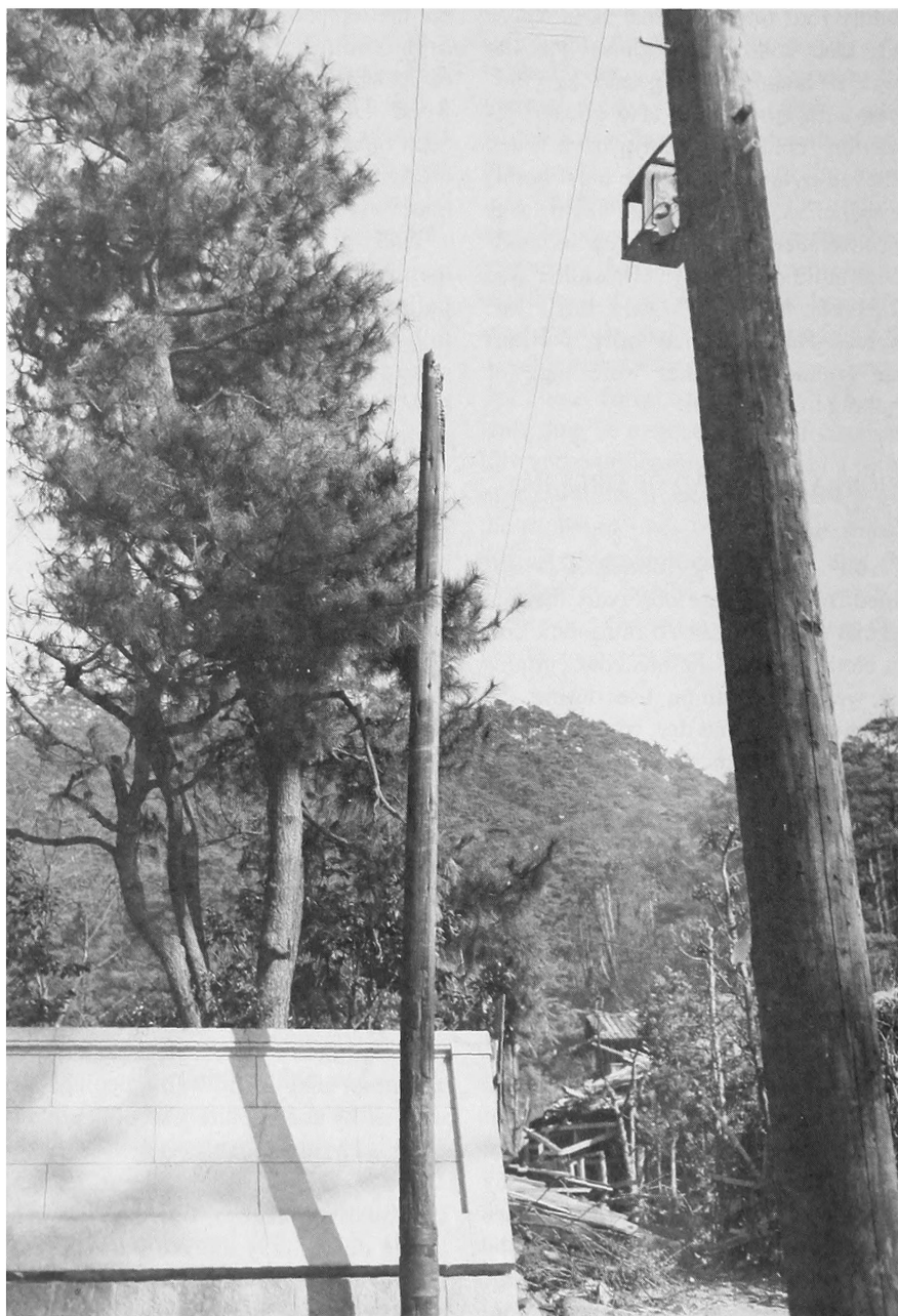
Figure 7.63. The top of a wood pole was reported as being ignited by the thermal radiation (1.25 miles from ground zero at Hiroshima, 5 to 6 cal/cm 2 ). Note the unburned surroundings; the nearest burned building was 360 feet away.
